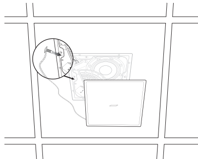
Figure 2. Insert safety lanyard pin.
